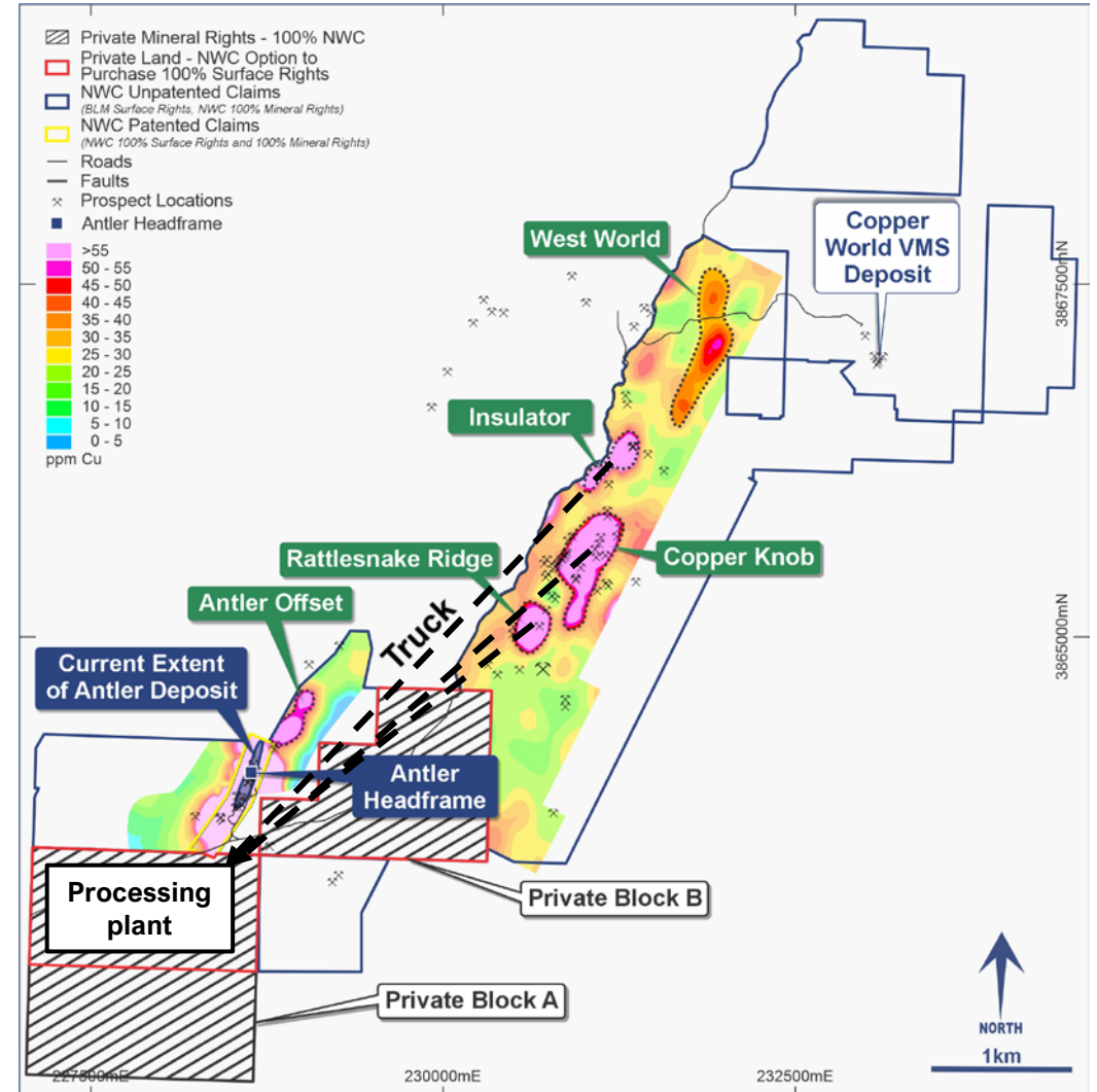
Plan View – Copper in Soil Geochemistry
